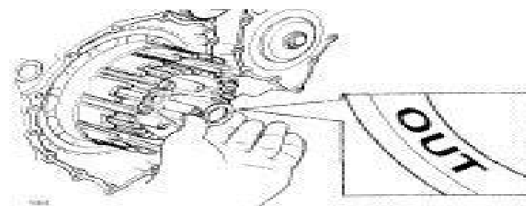
Belleville Washer 'Out' Mark
