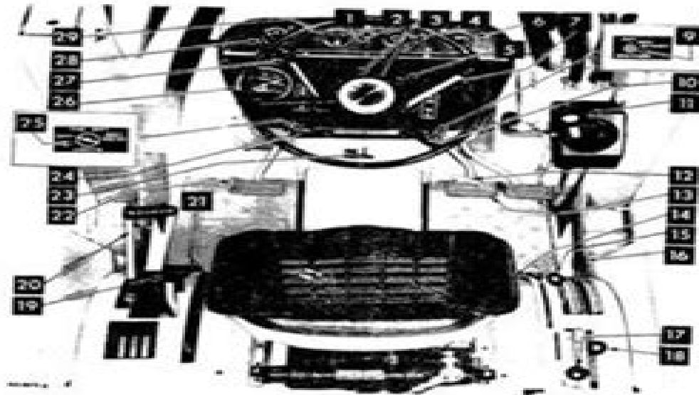
Location of instruments and controls facing toward loader end. (Synchronesh transmission with clutch pedal, and transmission speed and range levers.)
