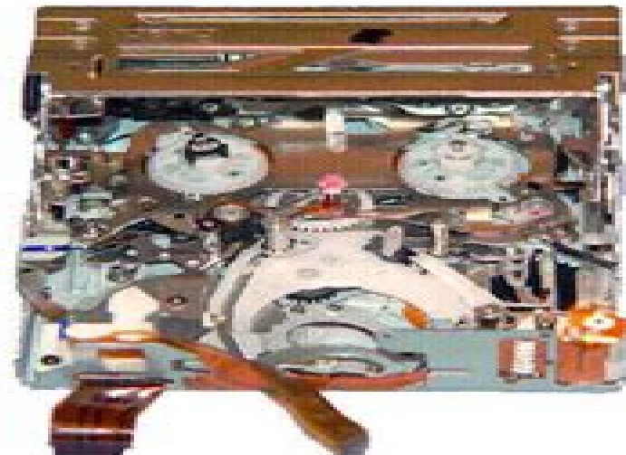
FIGURE 11-B - MECHANISM OPEN
