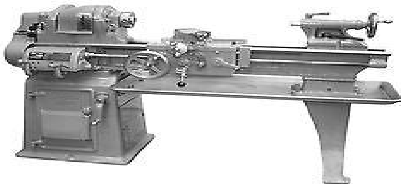
14" Industrial Lathe - Double Tumbler Gearbox
