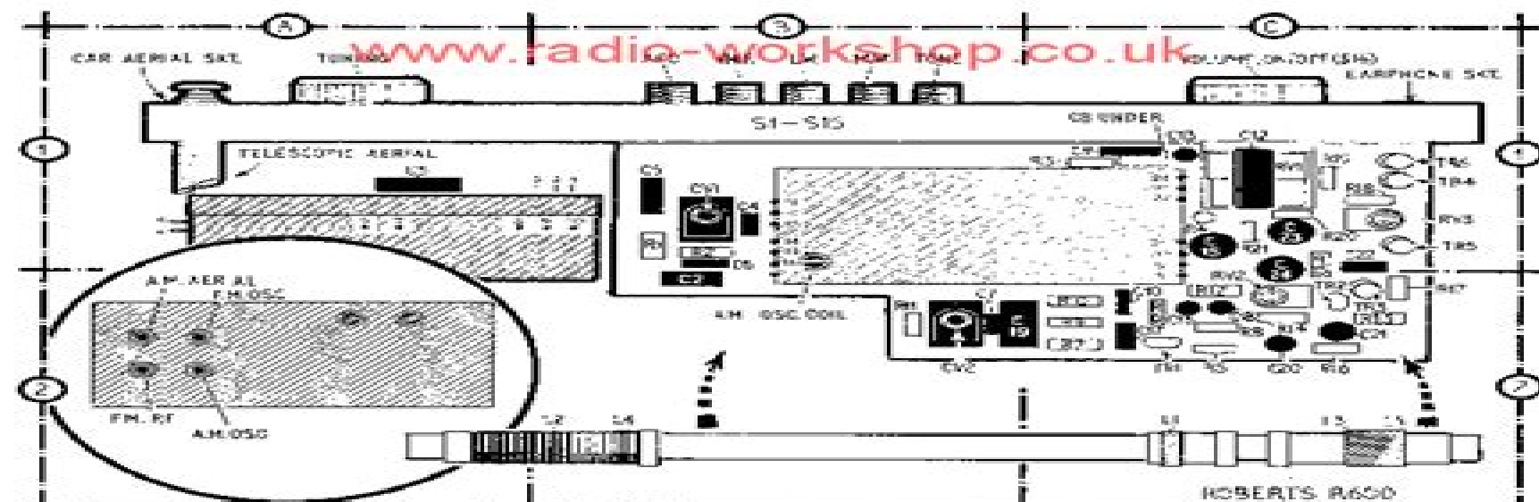
Component-side view of the printed panel as seen with the chassis removed from case.
