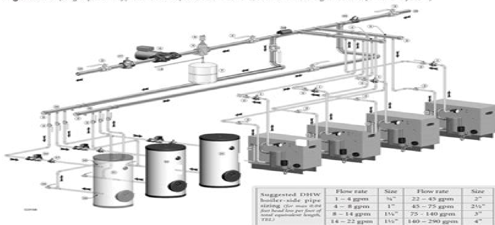
Figure 34 Piping layout — typical for multiple GV90+ boilers, with DHW storage heaters (4-boiler system)
