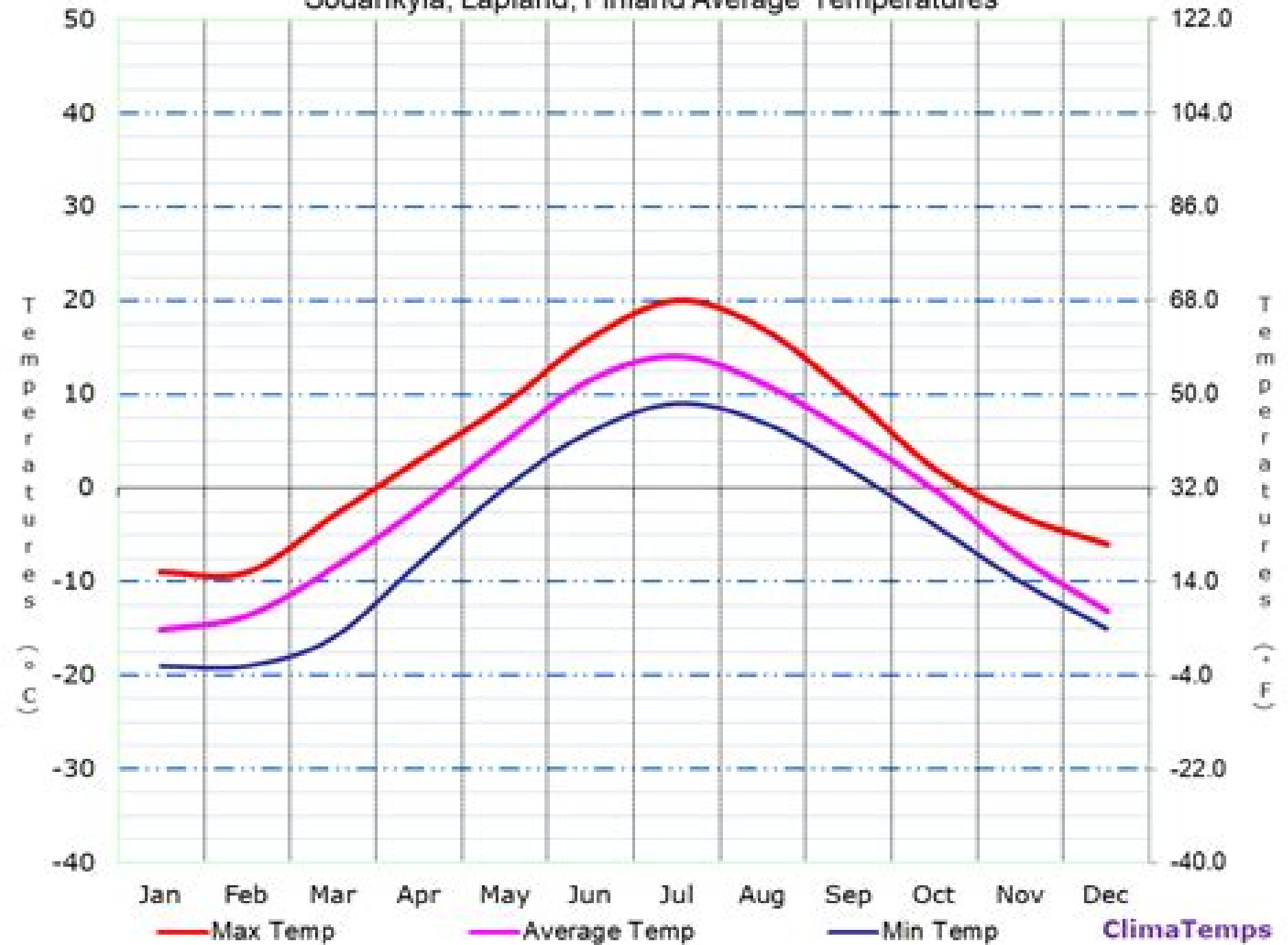
Sodankyla, Lapland, Finland Average Temperatures
