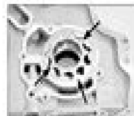
17.4 Note that the rollers 14 with the painted dots (arrowed) facing the oil pump cover - 1.4 litre engine
