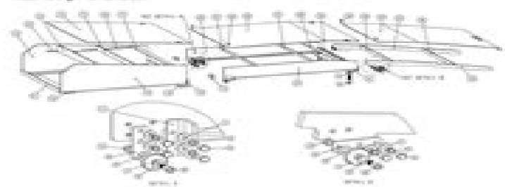
Figure 82 - Ramp Parts Map
