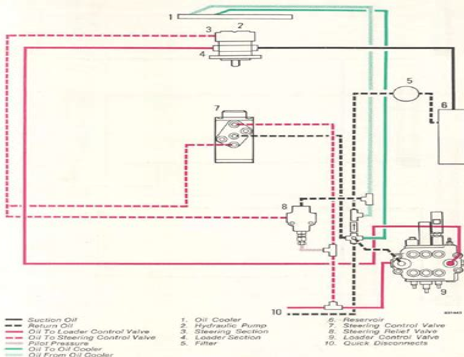
Hydraulic Diagram, Reservoir to Loader Control Valve and Connections for Rear Attachment
