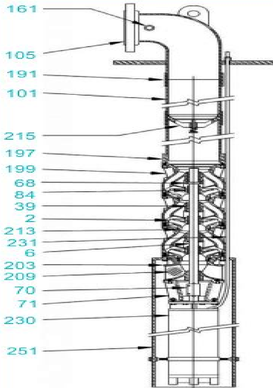
Vertical, Multistage, Submersible Pump
