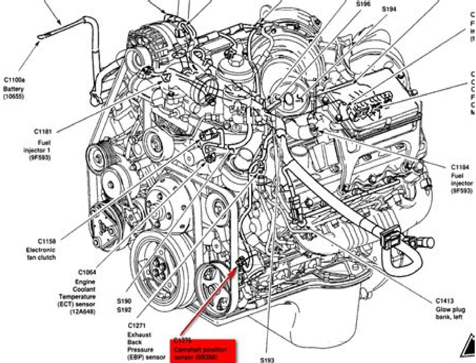
5.0L Diesel engine, LH side
