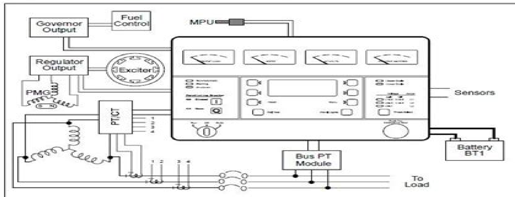
FIGURE 1-1. GENERATOR SET CONTROL FUNCTIONS
