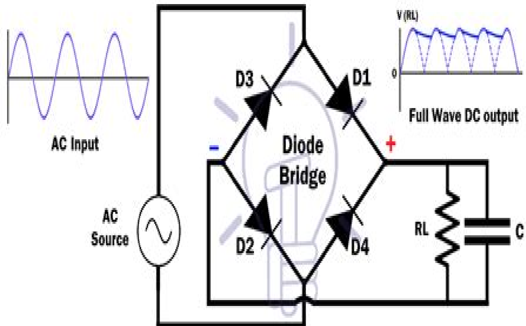
Bridge Rectifier Output With Capacitor
