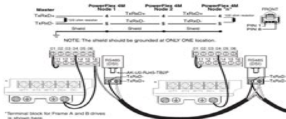
Figure C.1 Network Wiring Diagram
