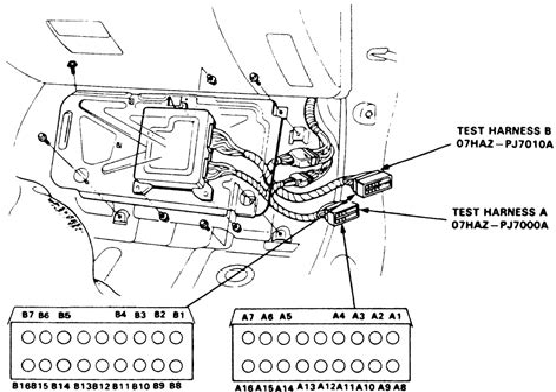
TERMINAL LOCATION
