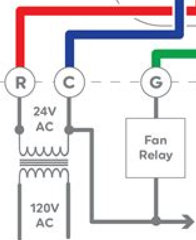
Indoor Handler Connections
