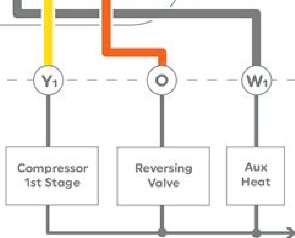
Heat Pump Connections
