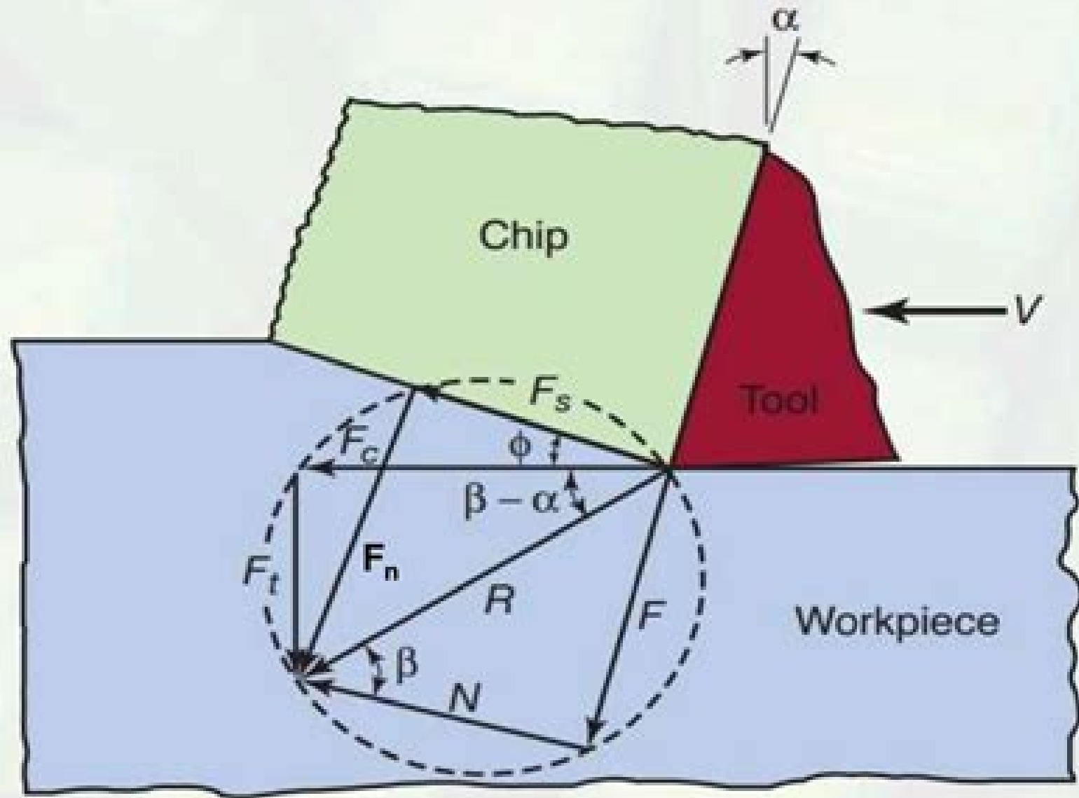
Force circle to determine various forces acting in the cutting zone.
