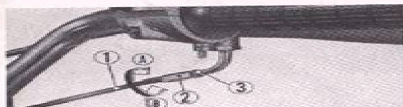
① Throttle cable ② Throttle cable adjust nut "A" ③ Lock nut ④ Decrease ⑤ Increase
