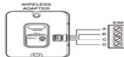
Fig. 6. THM4000R1000 Wireless Adapter wired to the EIM.
