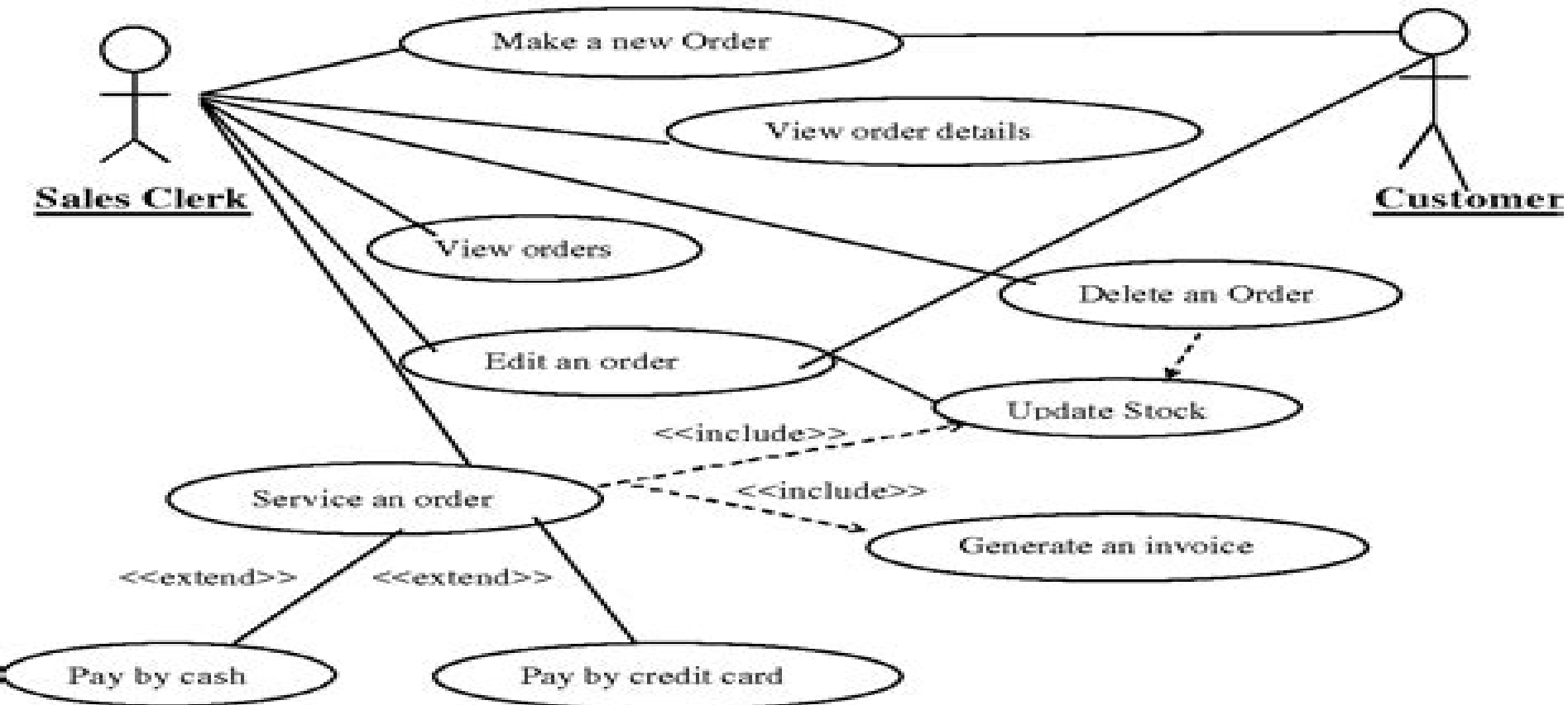
Figure 1.c. Use Case diagram for the order management subsystem
