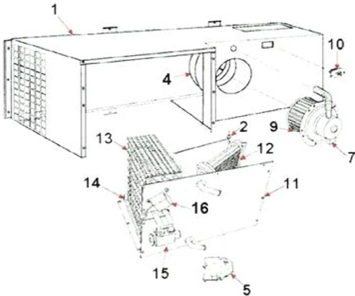
2011 KNI HVAC - A/C, Dash Unit (NEW)
