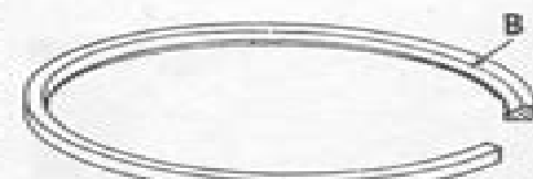
Fig. SK5-14—Install piston rings with bevel (B) to top.
