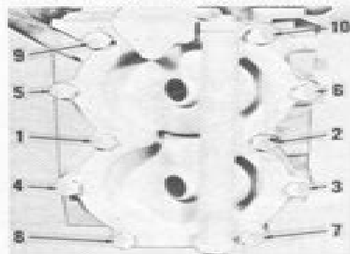
Fig. SK5-10—Cylinder head cap screws should be tightened in the sequence shown above.
