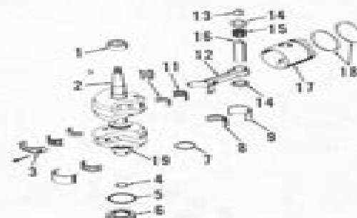
Fig. SK5-11—Exploded view of crankshaft assembly.
